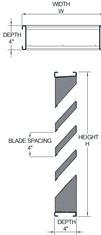
MODEL: ACL440 FRAME: CHANNEL FRAME DUCT-MOUNT (DM)
