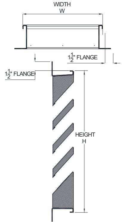
MODEL: ACL445 FRAME: CHANNEL FRAME DUCT-MOUNT (DM)
